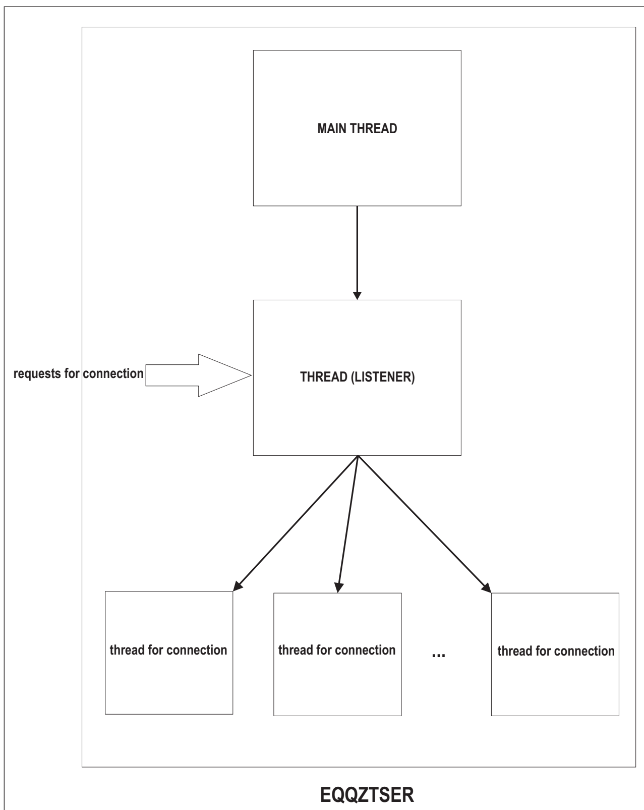
Figure 6. Internals of the EQQZTSER process.
