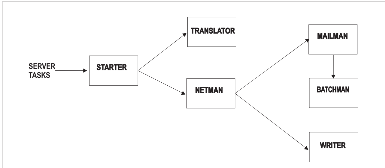
Figure 7. Tivoli Workload Scheduler for z/OS server processes for end-to-end scheduling with fault tolerance capabilities
