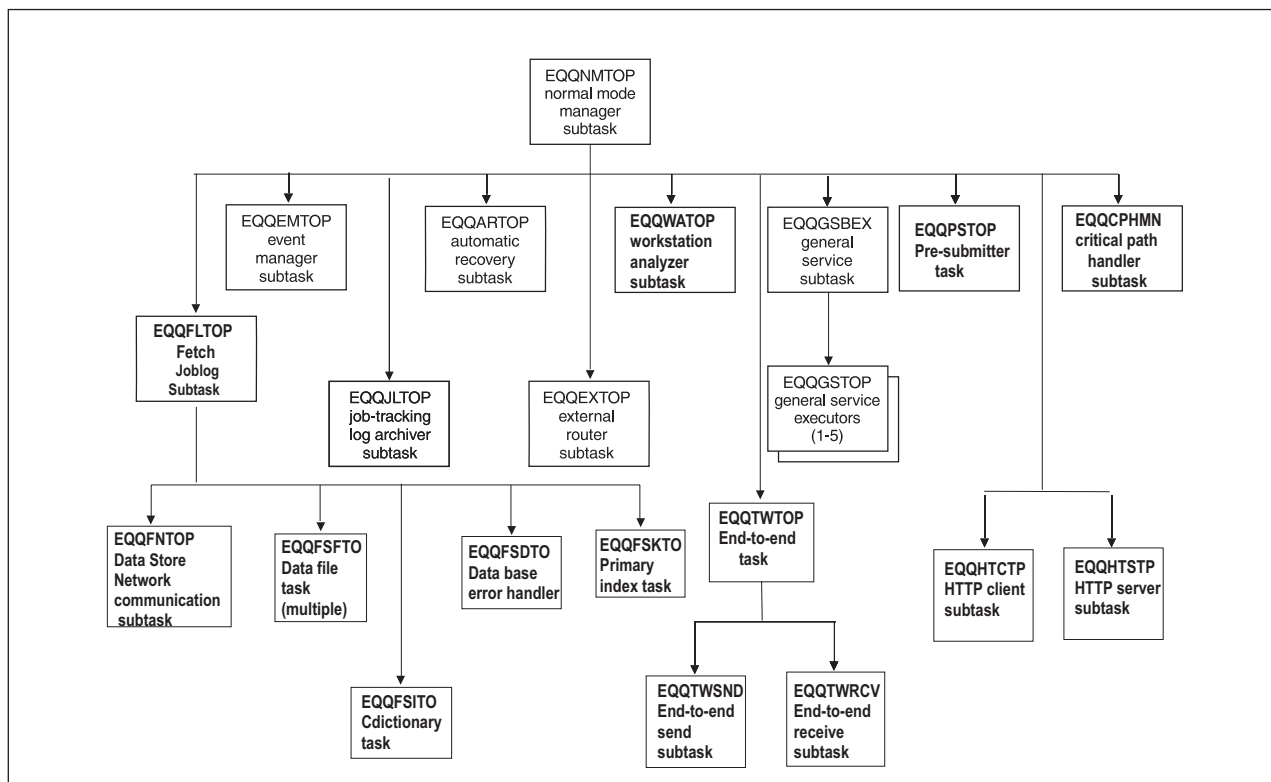
Figure 4. controller subtasks
